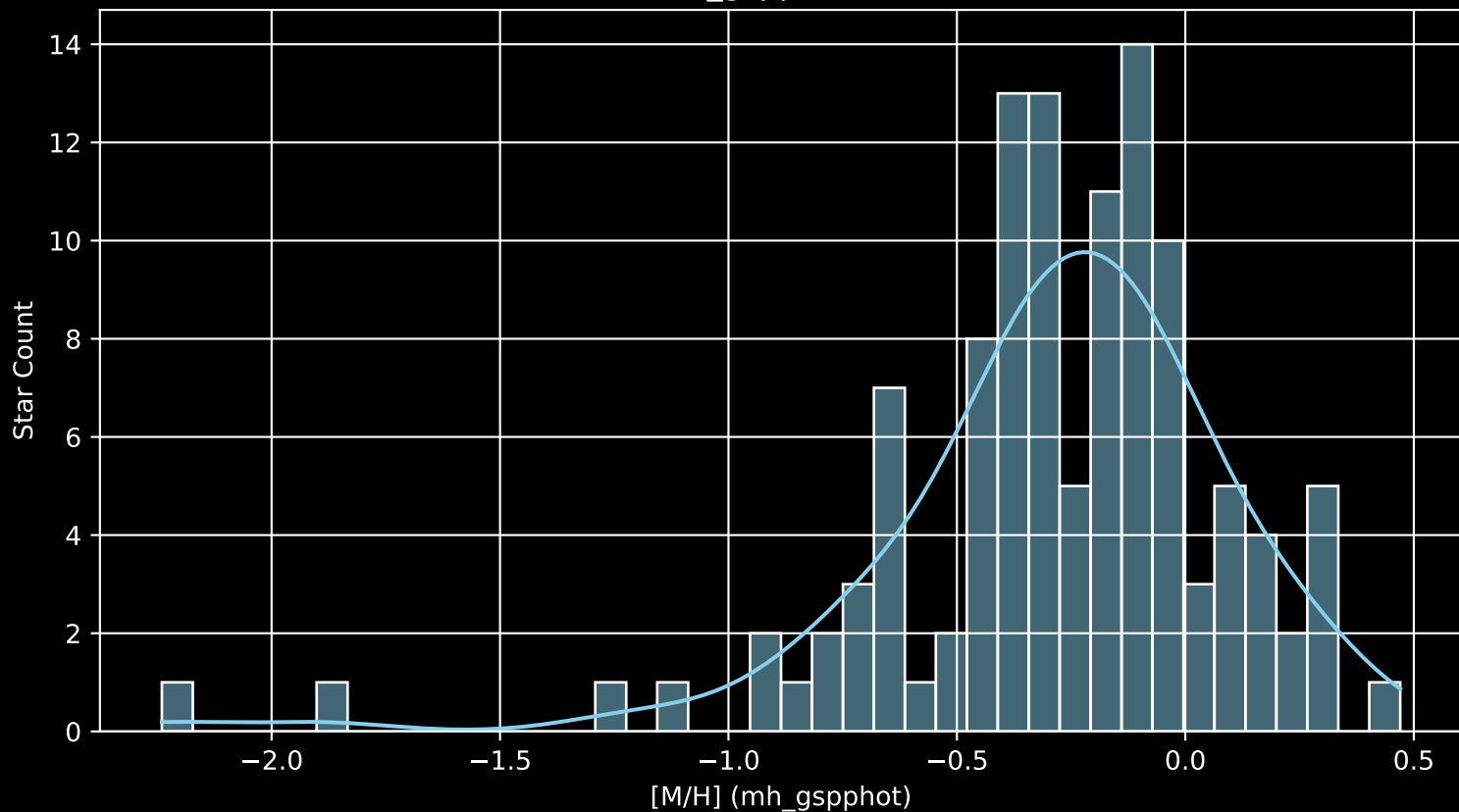
APOGEE DR17 Field: [061-25_MGA [M/H] (mh_gspphot) (n= 116)
