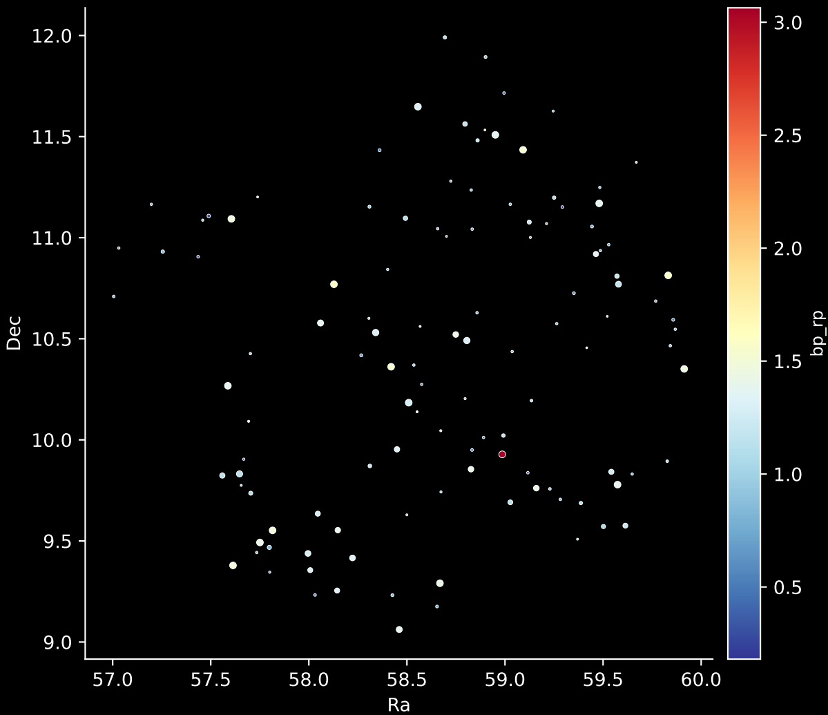
APOGEE DR17 Field: [061-25_MGA] Stars: 118
