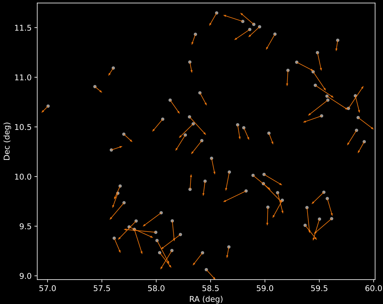
APOGEE DR17 Cluster 2 Proper Motion Vectors (n=71)
