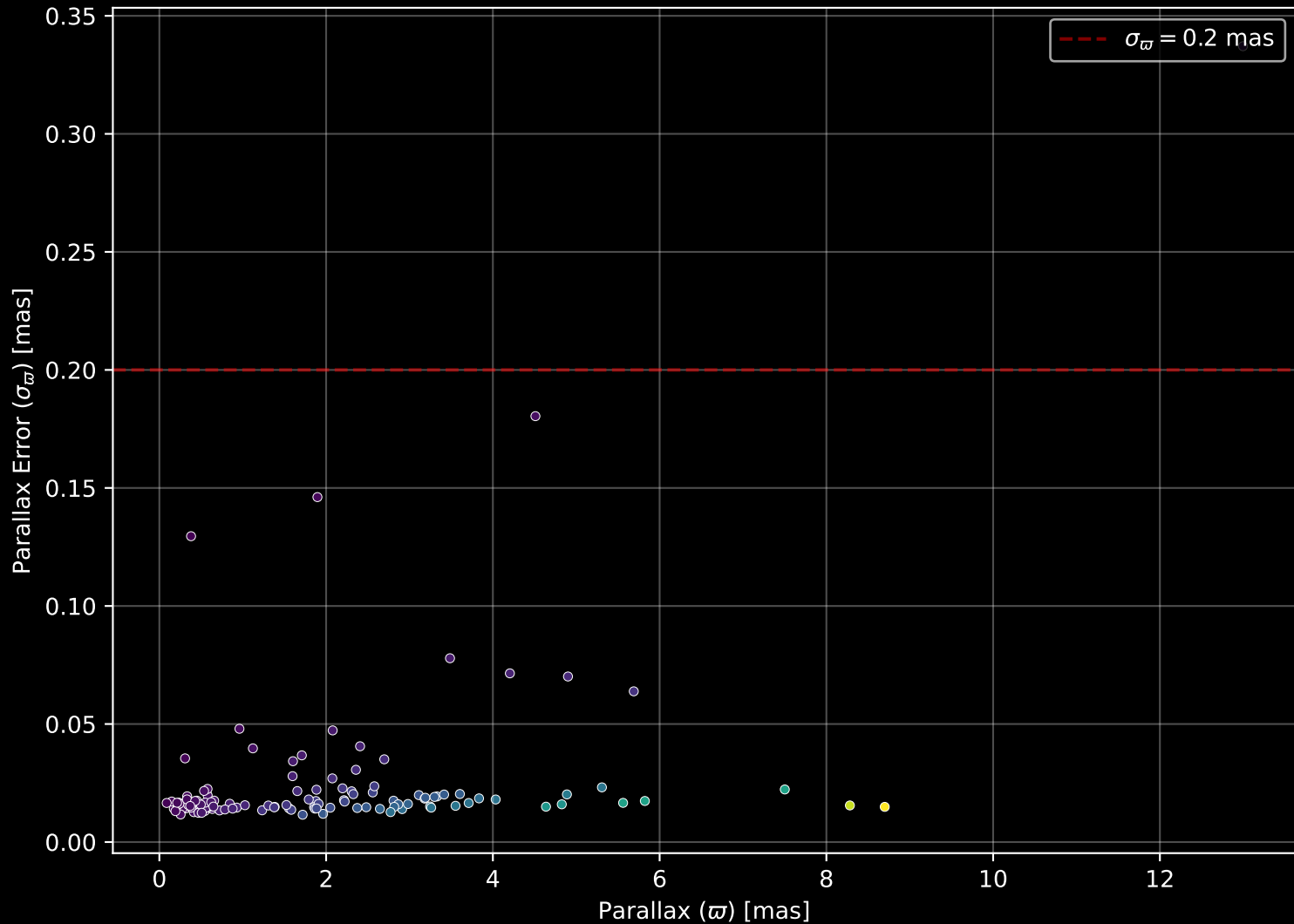
APOGEE DR17 Field: [061-25_MGA] Parallax Quality (n= 118)
