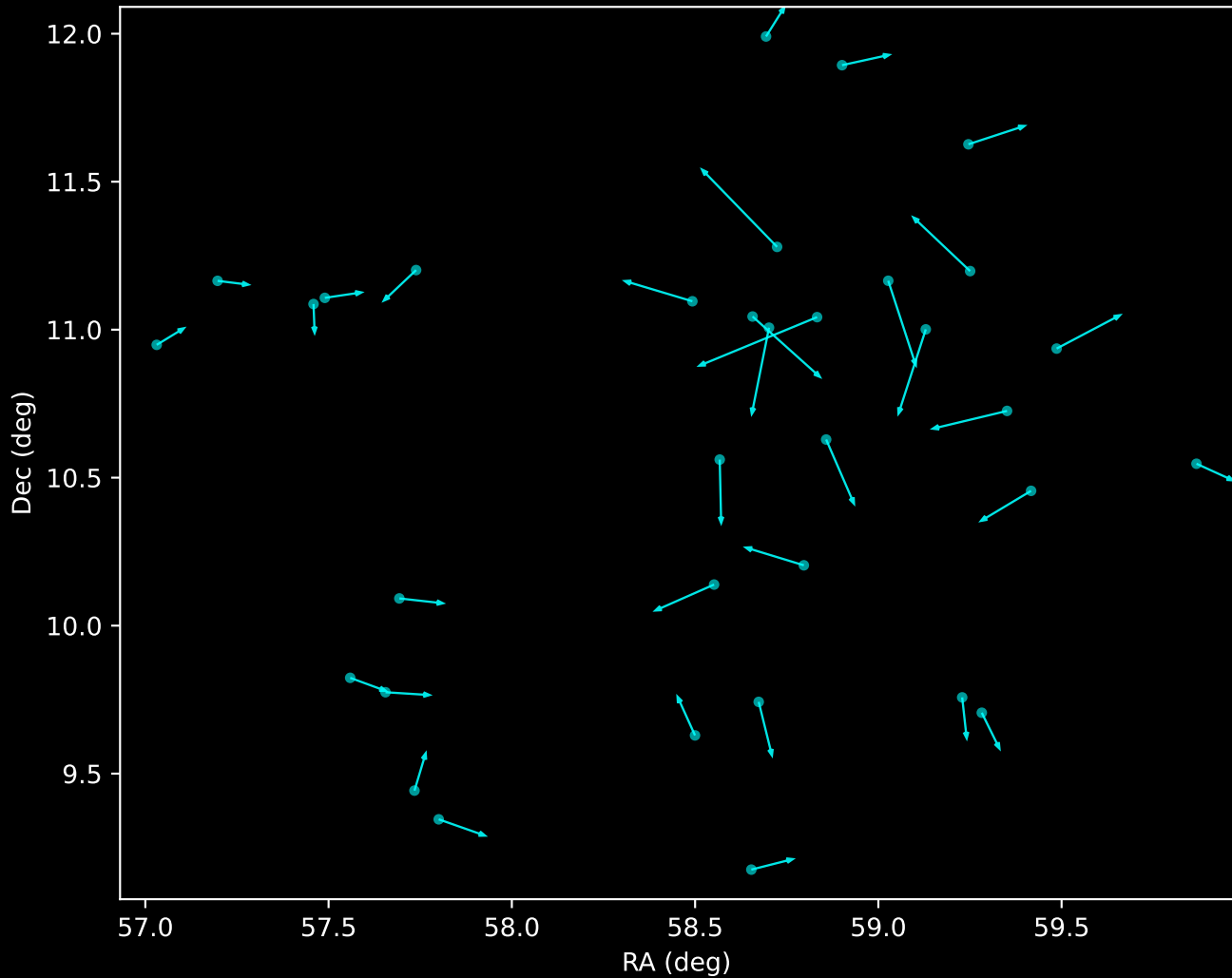
APOGEE DR17 Noise Stream Proper Motion Vectors (n=34)
