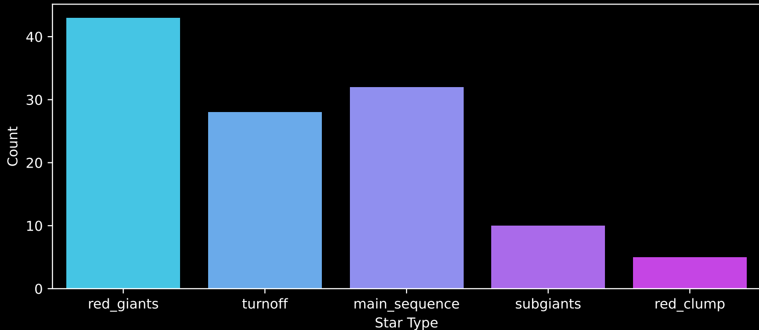
APOGEE DR17 Field: [061-25_MGA] Count plot of Star Type
