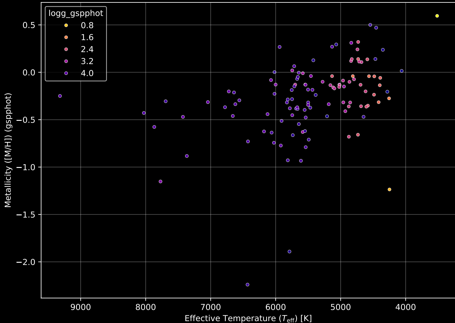
APOGEE DR17 Field: [061-25_MGA] Stellar Population Parameters (n= 118)
