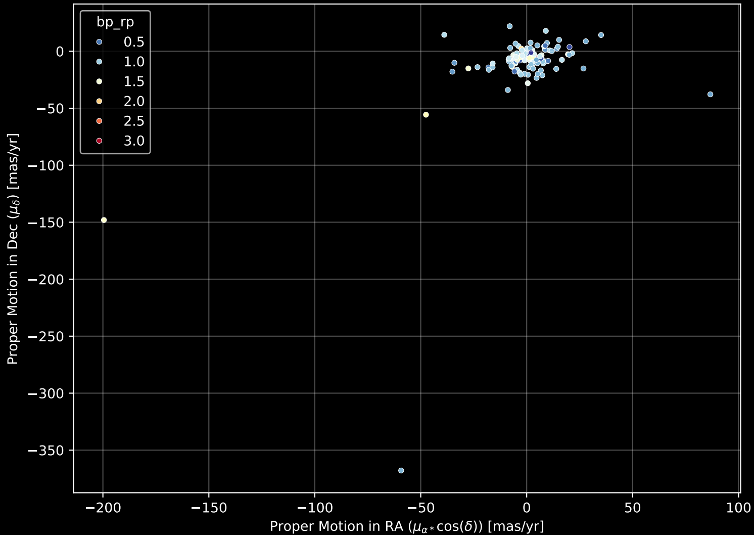
APOGEE DR17 Field: [061-25_MGA] Proper Motion Diagram (n= 118)
