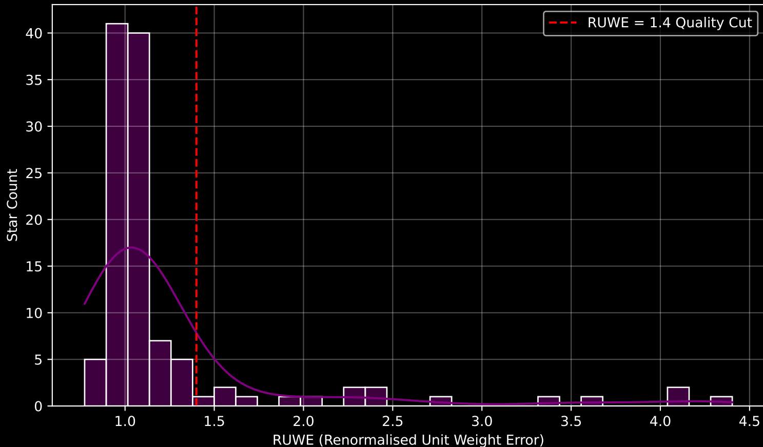
GAPOGEE DR17 Field [061-25_MGA] RUWE Distribution (n= 114)
